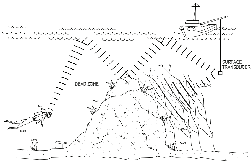
FIGURE 11: Communication through indirect and direct paths. Note kelp scattering sound. Without surface and bottom bounce, the diver would lose communications.
